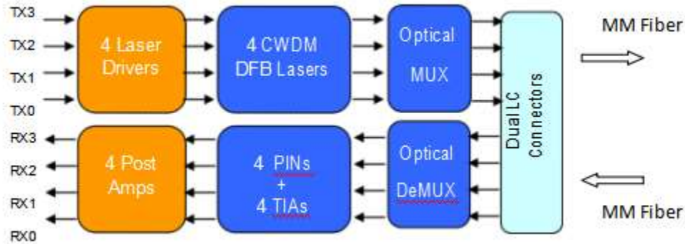
Figure1. Transceiver Block Diagram for Application over Multimode
